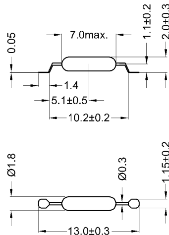
Dimensions (mm)
